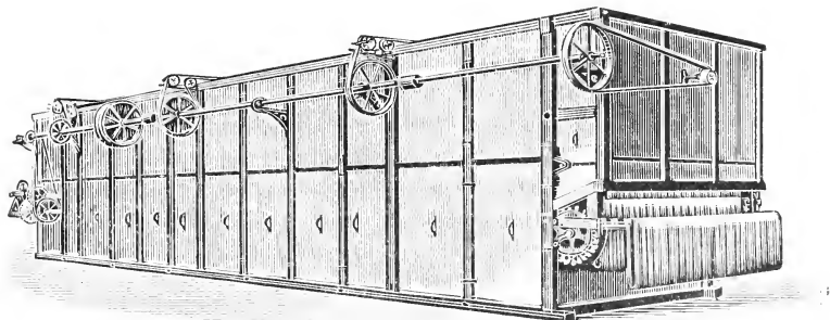
FIG. 41.—Automatic Yarn-dryer.
